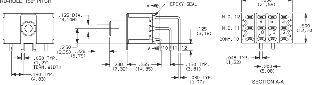
PC MOUNTING
